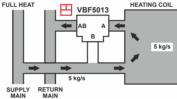
Fig. 10. Three-way mixing valve operation with coil bypass, full heat (not to scale)
