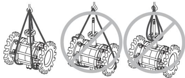
Fig. 1. Proper hoisting of VBF valves
