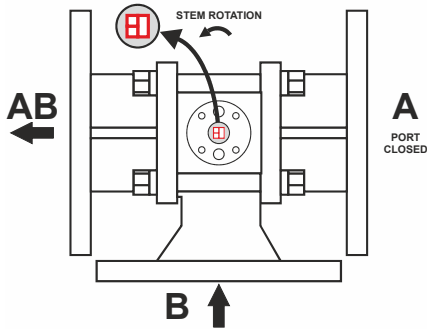
Fig. 9. Stem rotation, bypass flow
