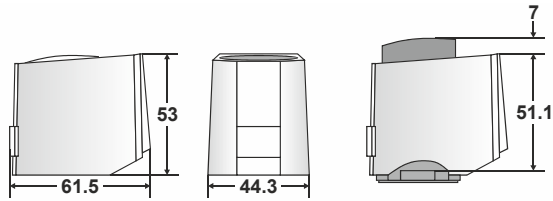
Fig. 1. Dimensions (in mm)
