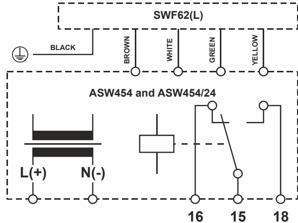
Fig. 4. Wiring diagram, ASW454 and ASW454/24
