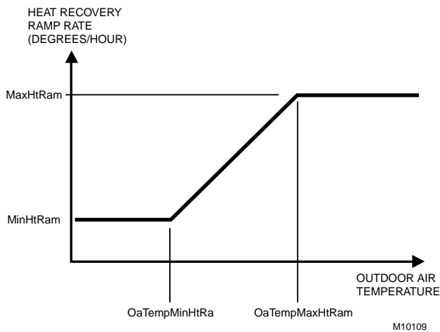
Fig. B-1. Setpoint ramping parameters with ramp rate calculation.
