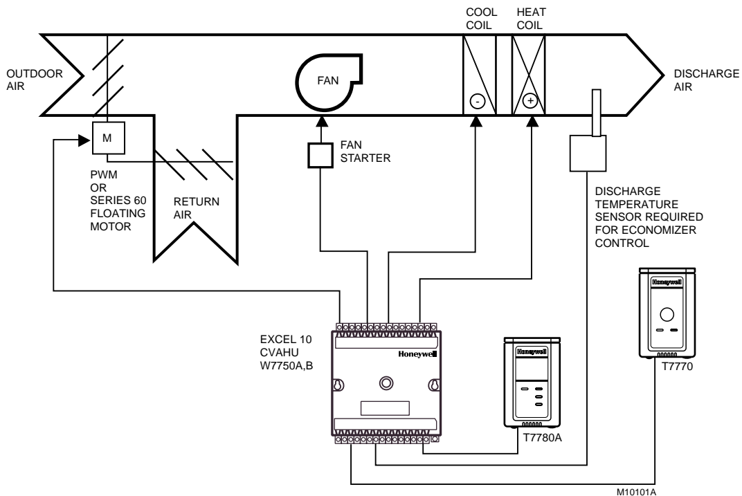
Fig. 15. Economizer control.
