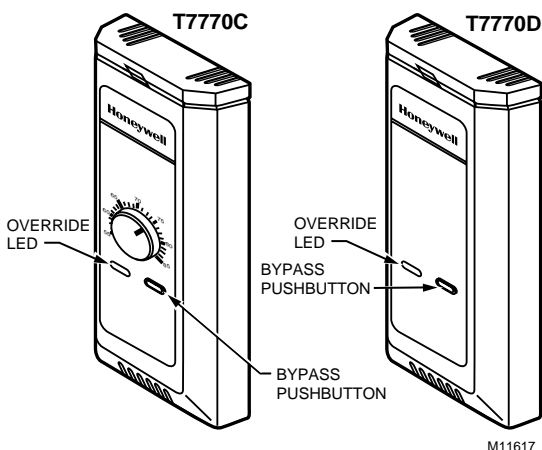
Fig. 39. The T7770C,D Wall Modules LED and Bypass pushbutton locations.
