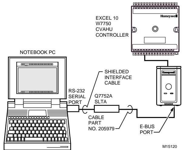
Fig. 17. Connecting the portable operator terminal to the E-Bus.
