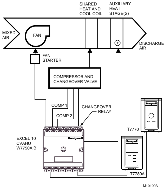
Fig. 14. Heat pump with two compressors and auxiliary heat stage(s).
