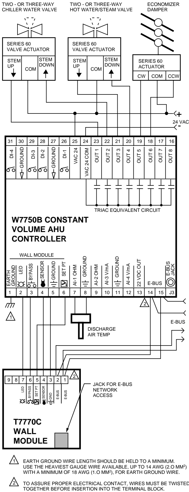
Fig. 29. W7750B Controller with floating heating, cooling and economizer wiring diagram. (For more information on note 2, refer to Fig. 24.)
