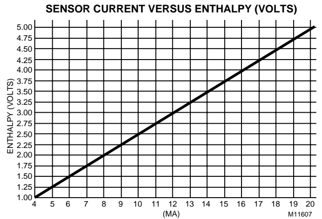
Fig. E-8. Graph of Sensor Current versus Enthalpy (volts).
