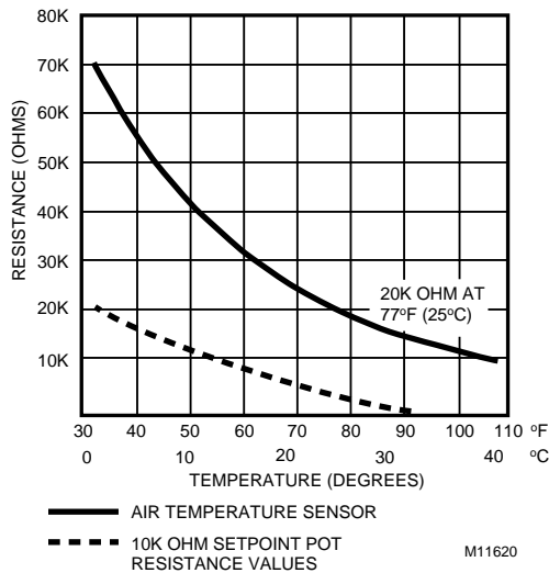
Fig. 36. Temperature sensor resistance plots.
