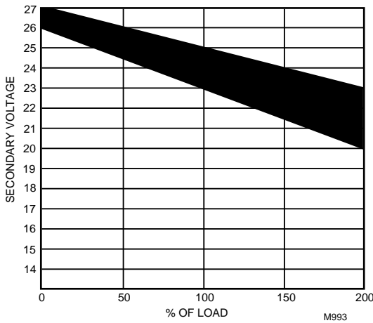
Fig. 20. NEMA class 2 transformer voltage output limits.
