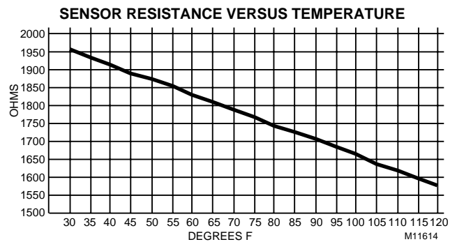
Fig. E-2. Graph of Sensor Resistance versus Temperature.
