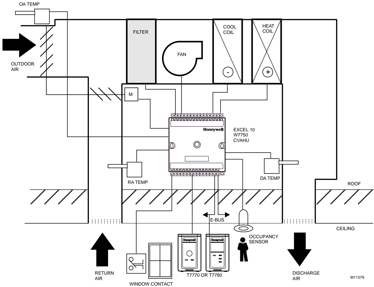
Fig. B-4. Schematic diagram for a typical W7750B Unit.
