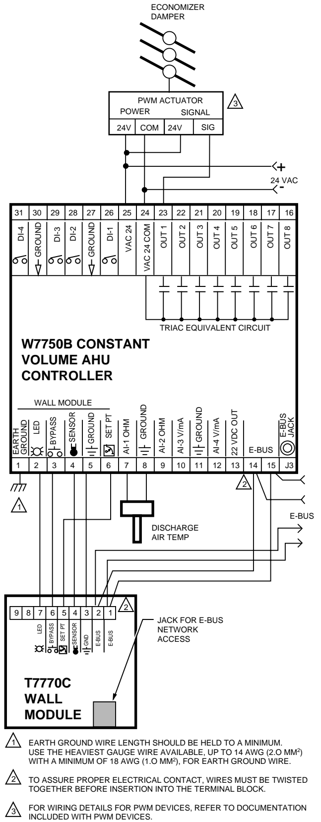
Fig. 30. W7750B Controller PWM damper actuator wiring diagram. (For more information on note 2, refer to Fig. 24.)
