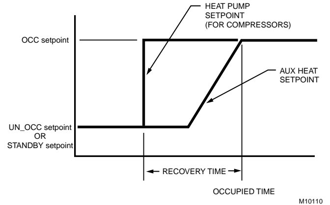
Fig B-2. Setpoint ramping parameters with setpoint calculation.
