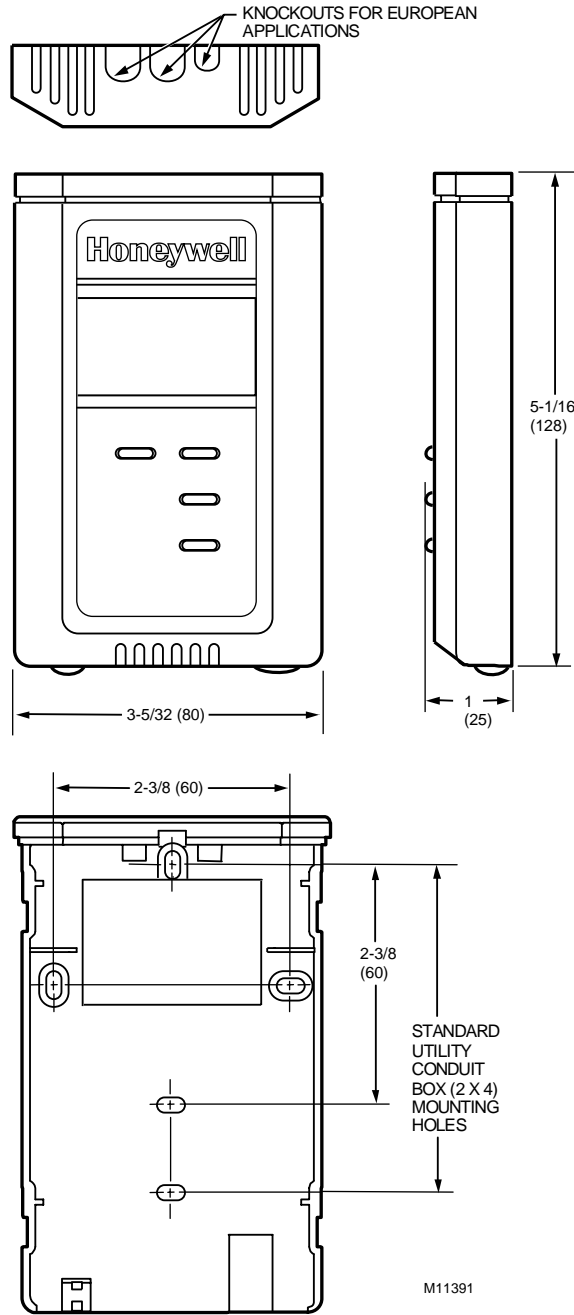
Fig. 10. T7780A construction in in. (mm).
