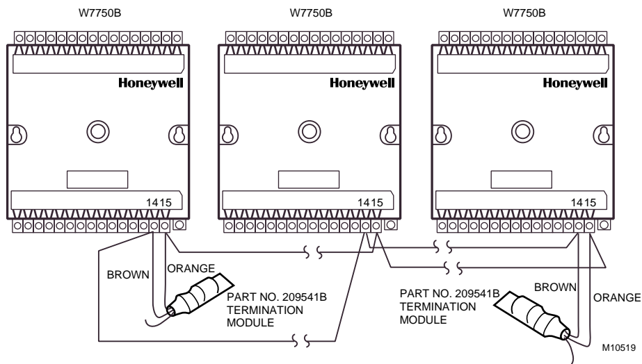
Fig. 34. Typical doubly terminated daisy-chain E-Bus segment termination module wiring diagram.
