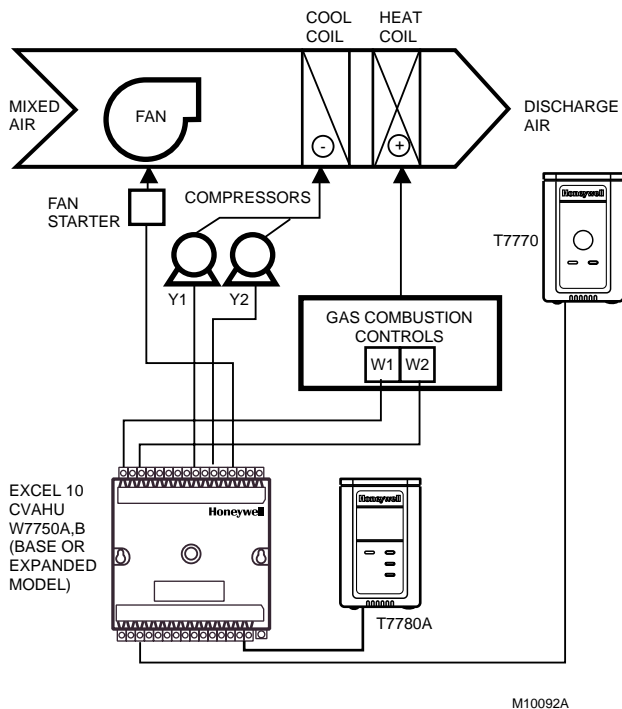
Fig. 12. Fan with two stages of heating and two stages of cooling.
