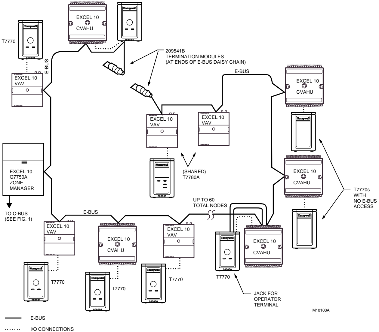
Fig. 18. Wiring layout for one doubly terminated daisy-chain E-Bus segment.
