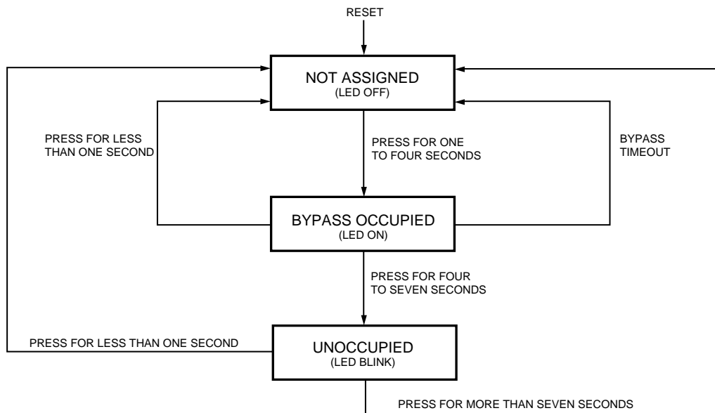
Fig. B-0. LED and Bypass pushbutton operation.
