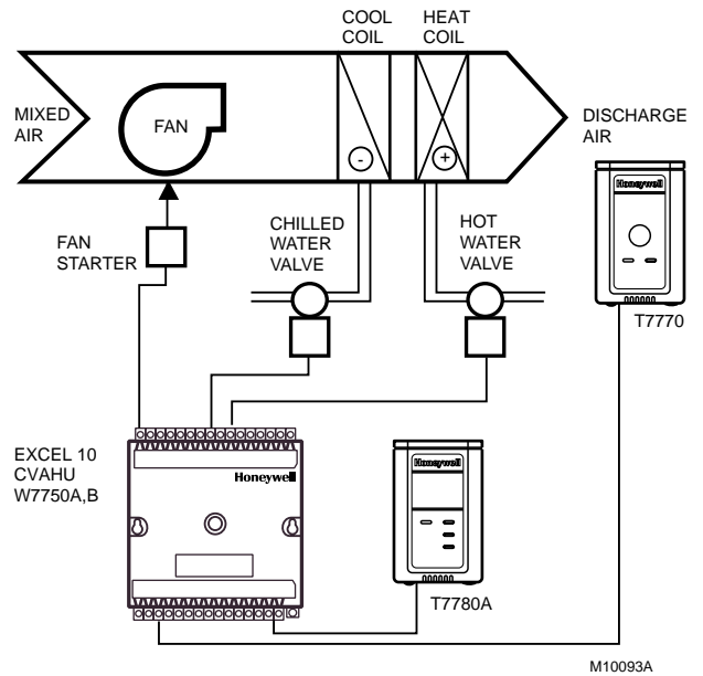
Fig. 13. Fan, modulating heating and modulating cooling.
