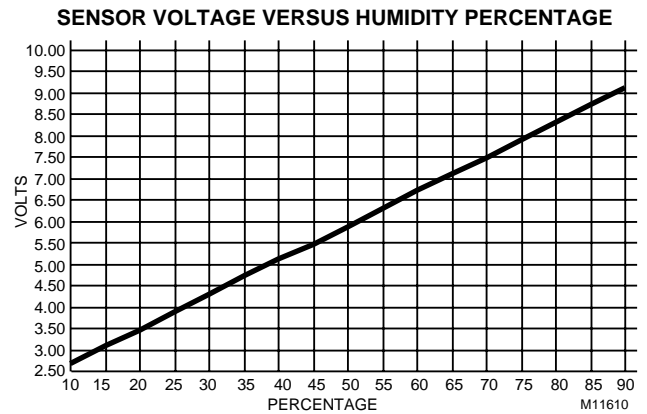
Fig. E-6. Graph of Sensor Voltage versus Humidity.
