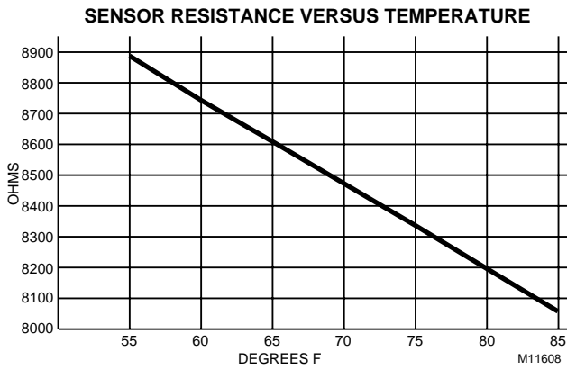
Fig. E-5. Graph of Sensor Resistance versus Temperature.
