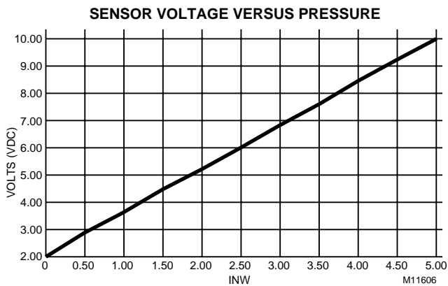
Fig. E-13. Graph of Sensor Voltage (Vdc) versus Pressure (Inw).
