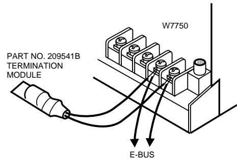
(B) Installing E-Bus Termination Module at W7750
