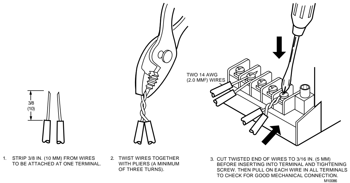
Fig. 24. Attaching two or more wires at terminal blocks.
