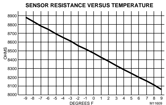
Fig. E-4. Graph of Sensor Resistance versus Temperature.
