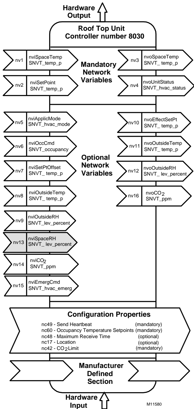
Fig. 8. Functional profile of LonMark® RTU object details (variables not implemented in Excel 10 CVAHU are greyed).
