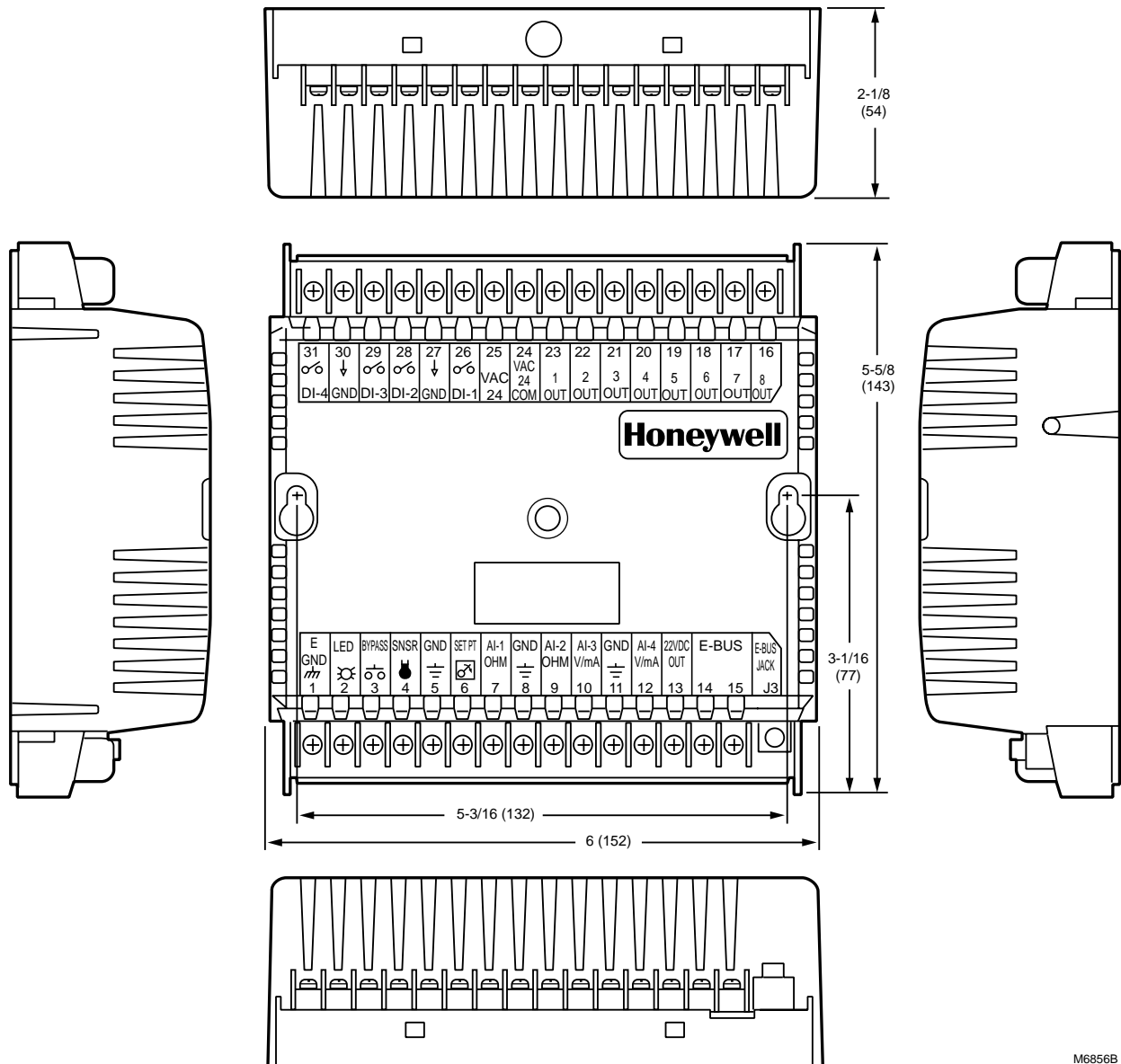
Fig. 6. W7750B construction in in. (mm).
