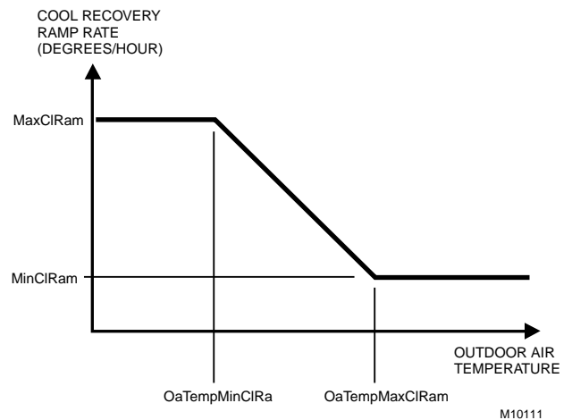
Fig. B-3. Setpoint ramping parameters with ramp rate calculation.
