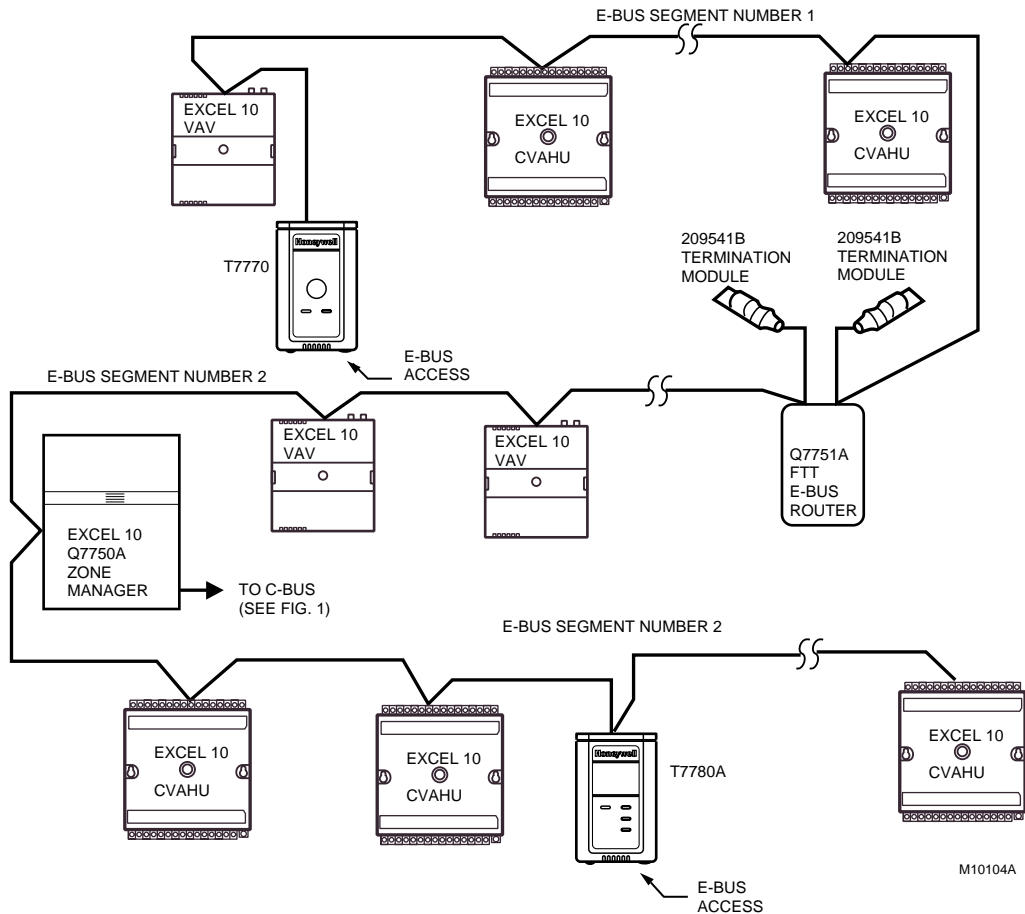
Fig. 19. Wiring layout for two singly terminated E-Bus segments.
