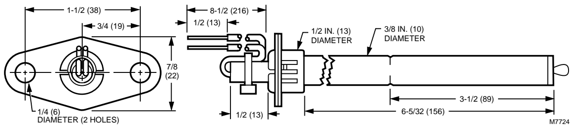
Fig. 11. C7770A construction in in. (mm).
