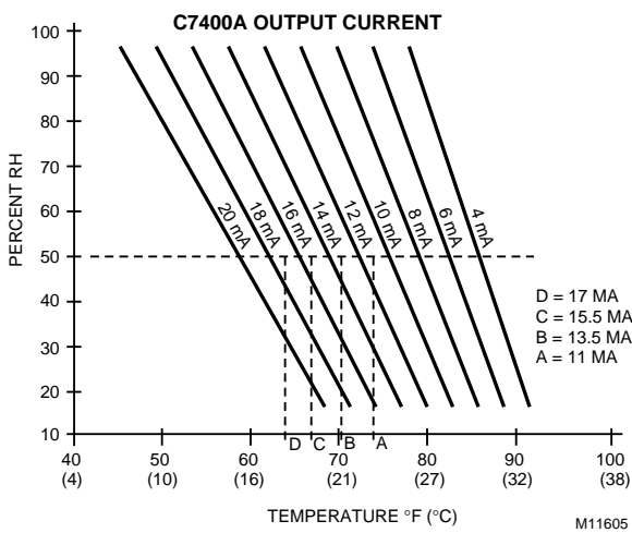
Fig. E-10. C7400A Solid State Enthalpy Sensor output current vs. relative humidity.
