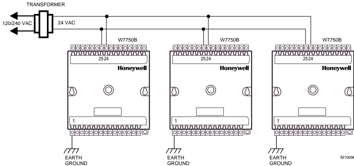
Fig. 22. Power wiring details for two or more Excel 10s per transformer.
