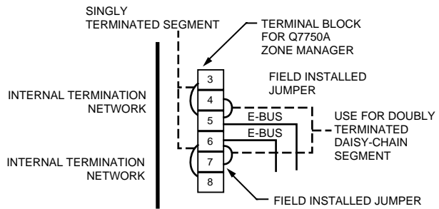
(A) Enabling Internal Termination Network using jumpers in the Q7750A Zone Manager
