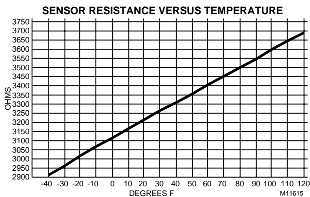
Fig. E-1. Graph of Sensor Resistance versus Temperature.
