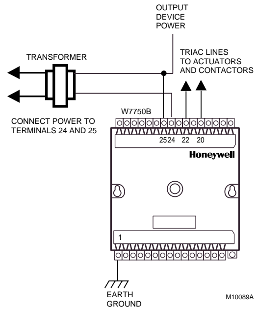
Fig. 21. Power wiring details for one Excel 10 per transformer.
